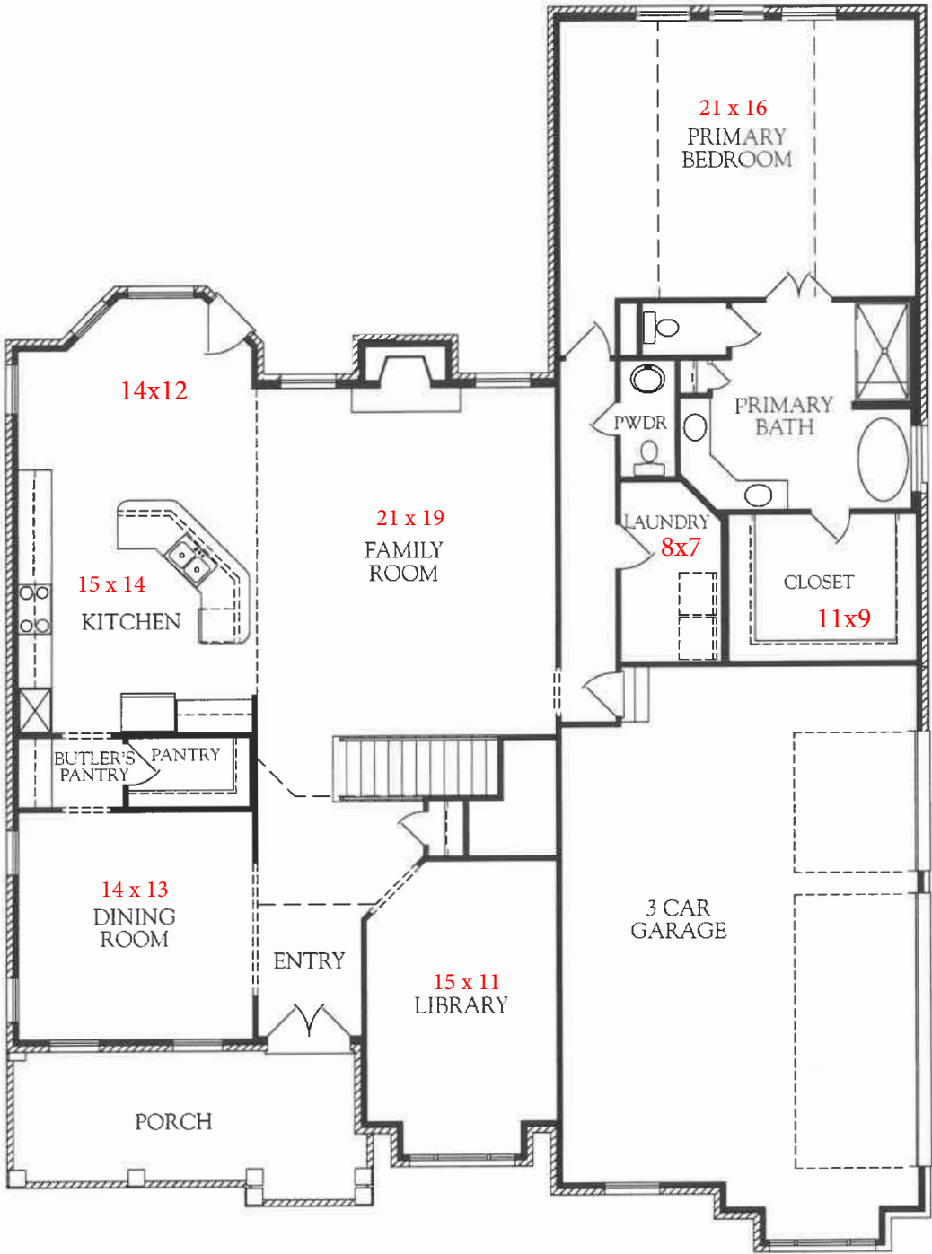
First Floor
